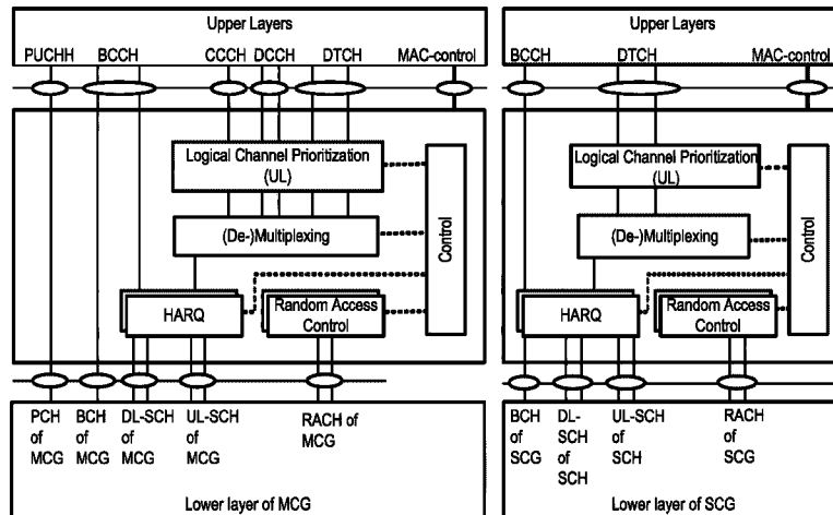
Dual-Connectivity-two MAC entities at UE side
