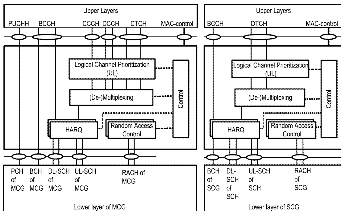
Dual-Connectivity- two MAC entities at UE side
