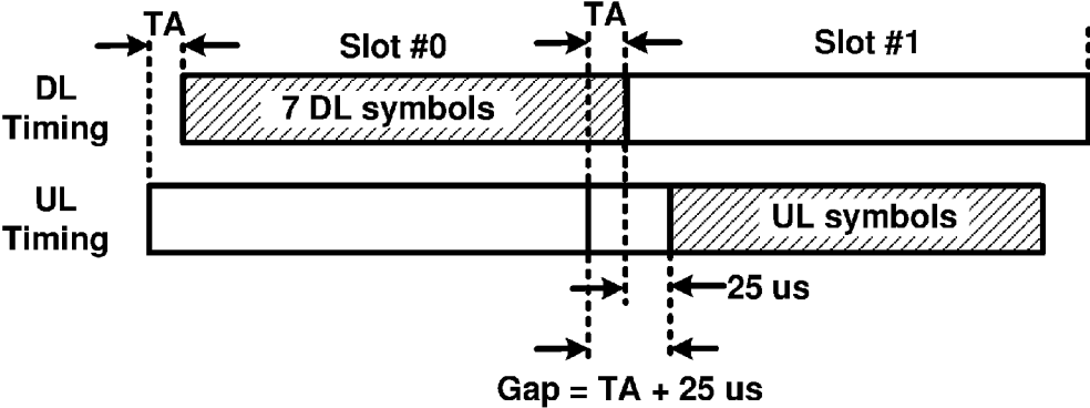
Example DL and UL Timing in a UE
