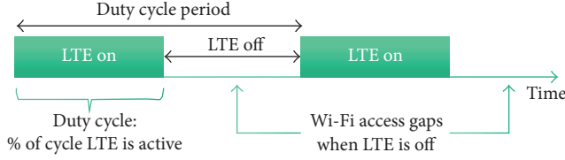
FIGURE 1: Air time sharing LTE-U.
